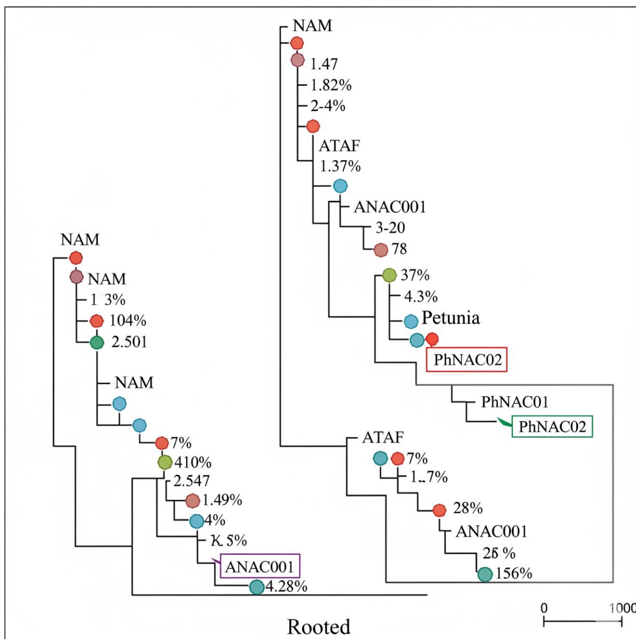
Figure 2 (Phylogenetic Tree)
